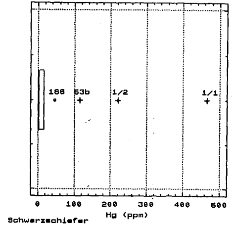
Box-and-Whisker Plot
