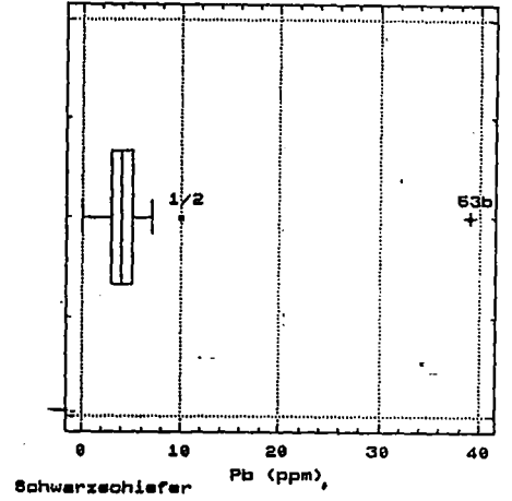
Box-and-Whisker Plot
