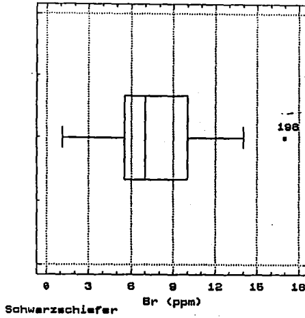
Box-and-Whisker Plot
