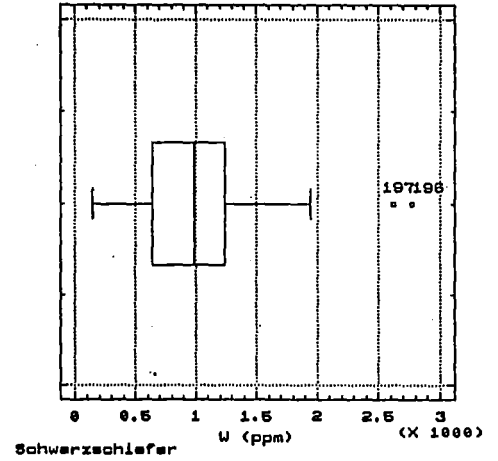
Box-and-Whisker Plot
