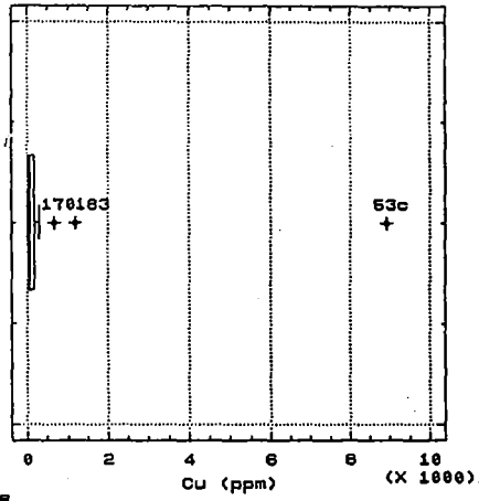
Box-and-Whisker Plot
