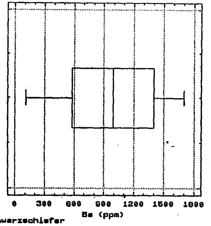
Box-and-Whisker Plot
